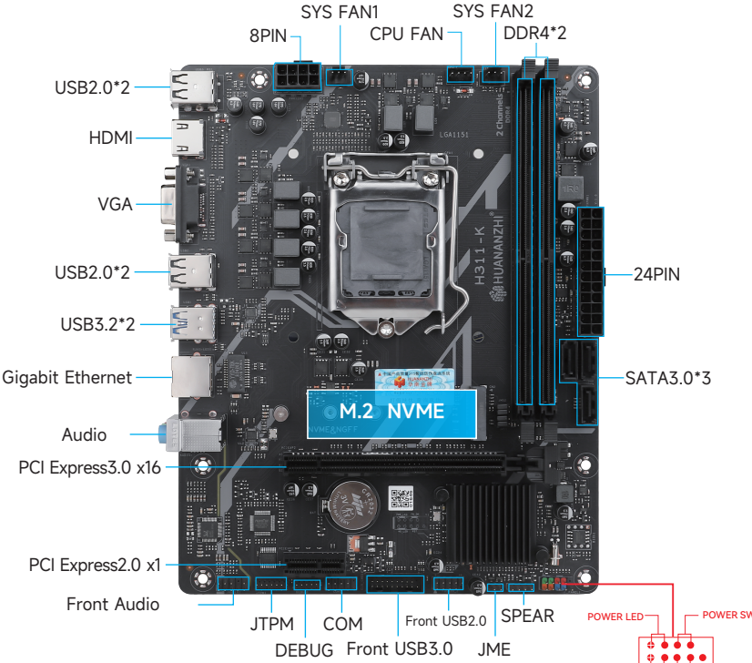
1-1 H311-K Motherboard Illustration
