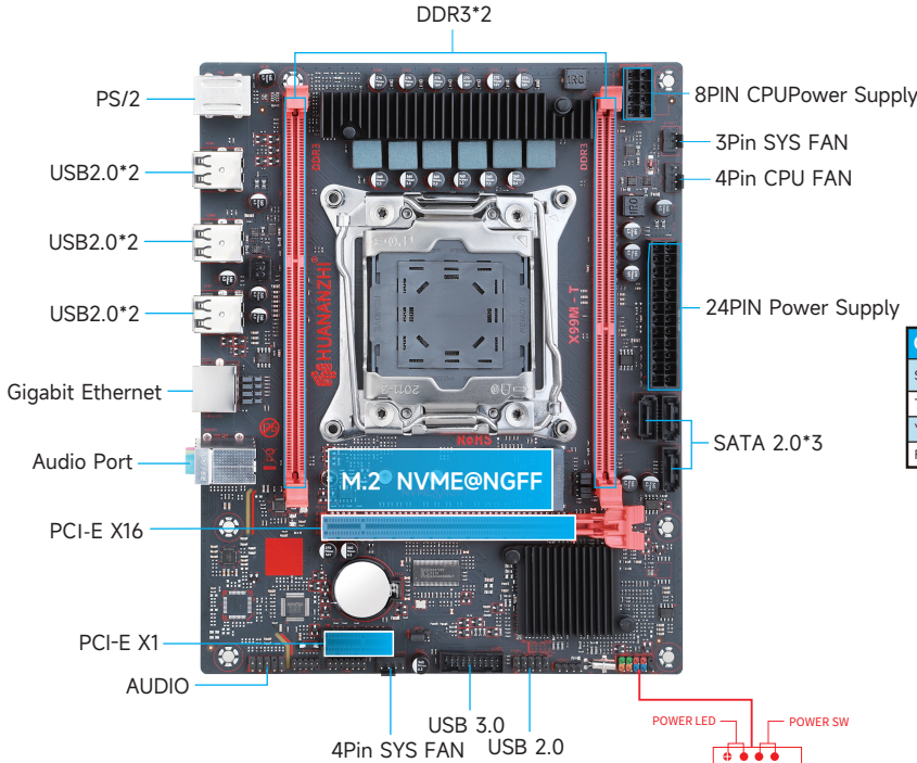
1-1 X99M-T Motherboard Illustration
