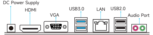
1-2 Overall Rear I/O Panel Display
