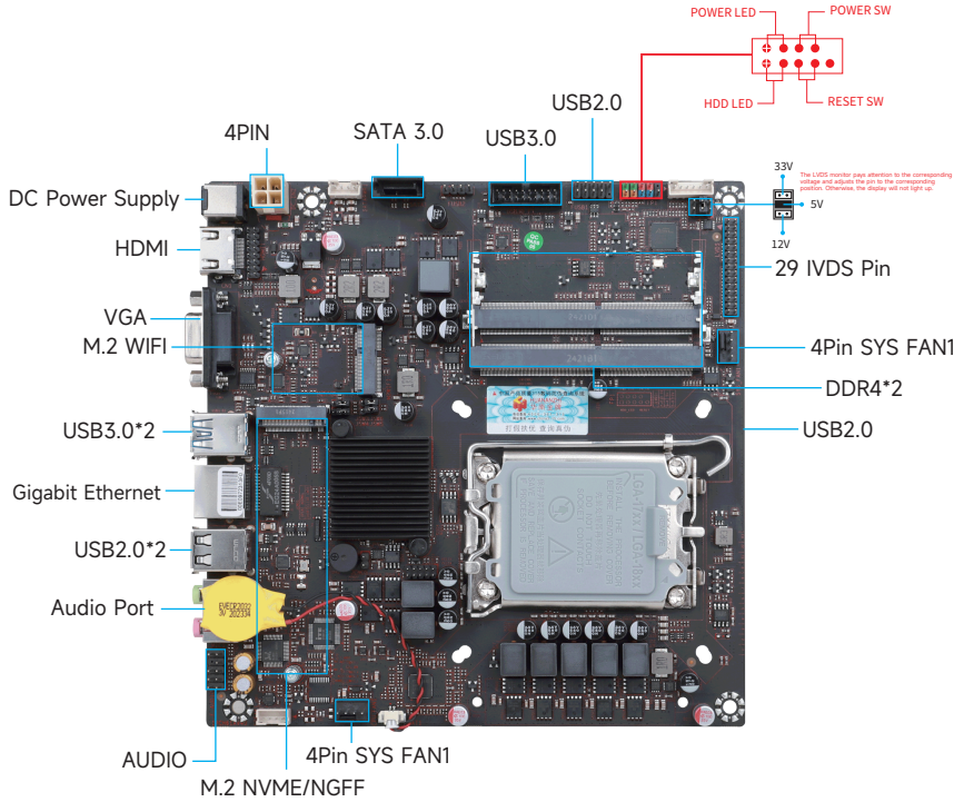
1-1 H610M-I Motherboard Illustration
