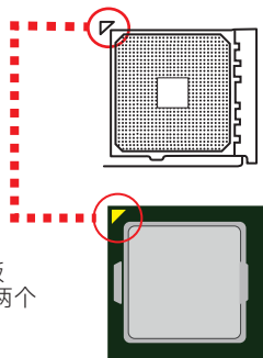
图2-5 CPU安装
