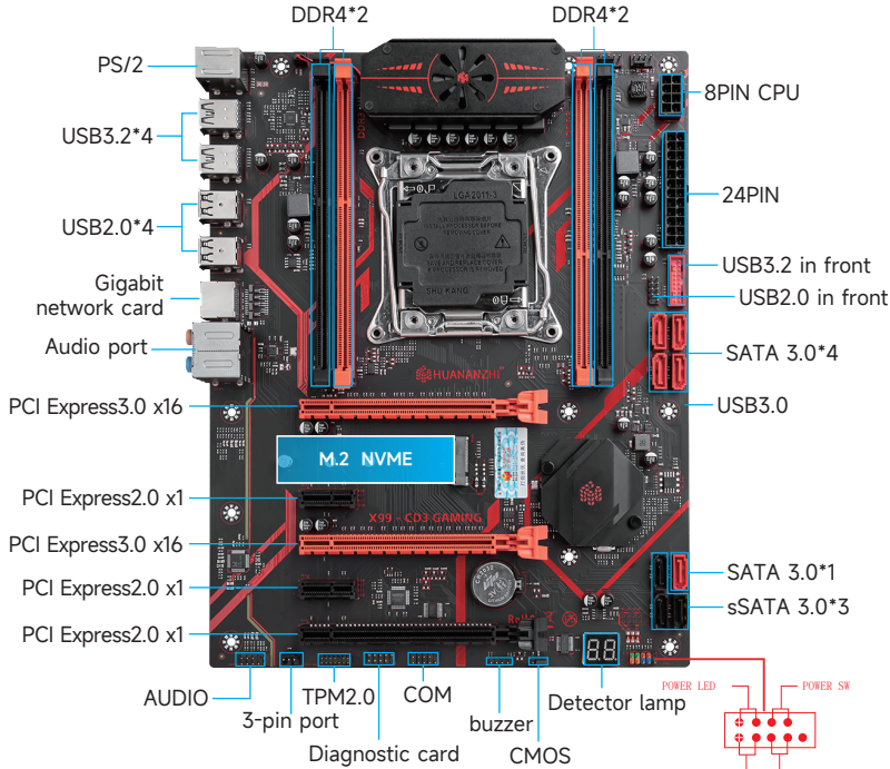
1-1 X99-CD3 GAMING Motherboard Illustration
