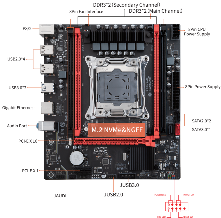
1-1 X79-4MT V2.0 Motherboard illustration
